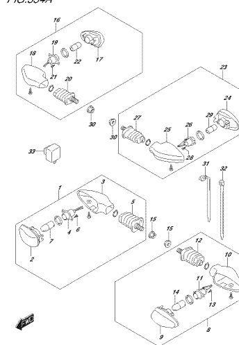
DOUBLE PPT 334A TURN SIGNAL LAMP
