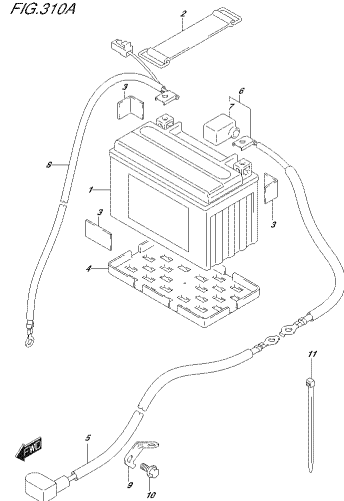
DOUBLE PPT 310A BATTERY
