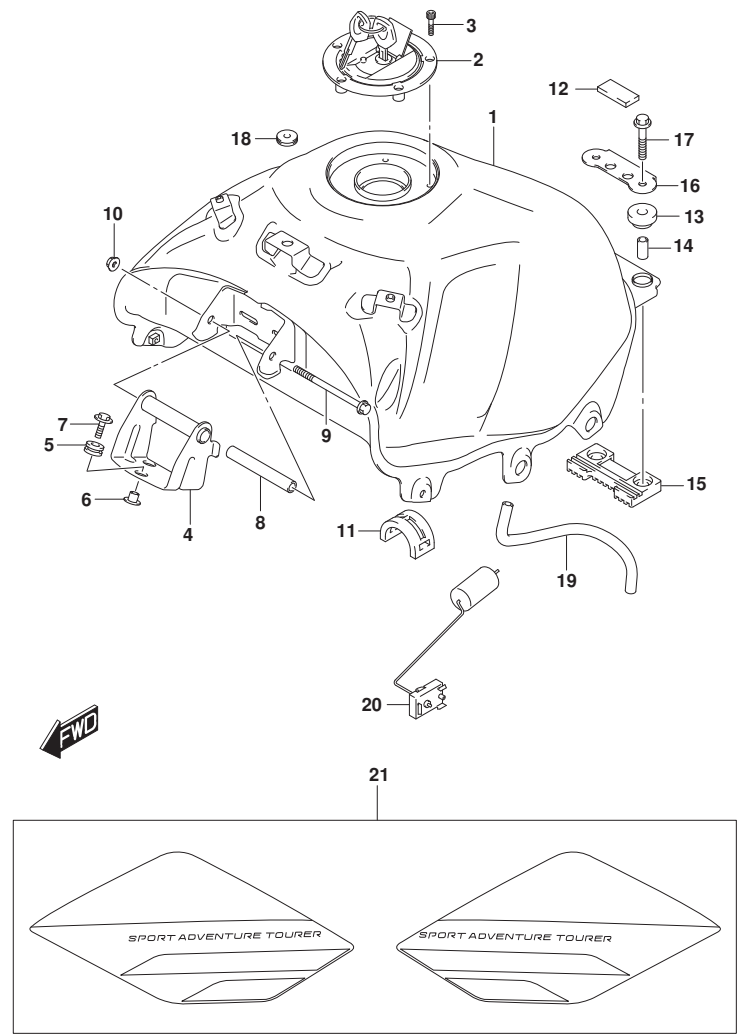
DL250L8_P71_420A FUEL TANK
