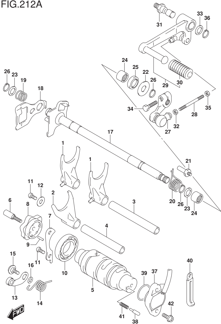
DL250L8_P71_212A GEAR SHIFTING
