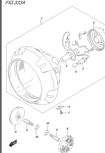
DOUBLE PPT 330A HEADLAMP
