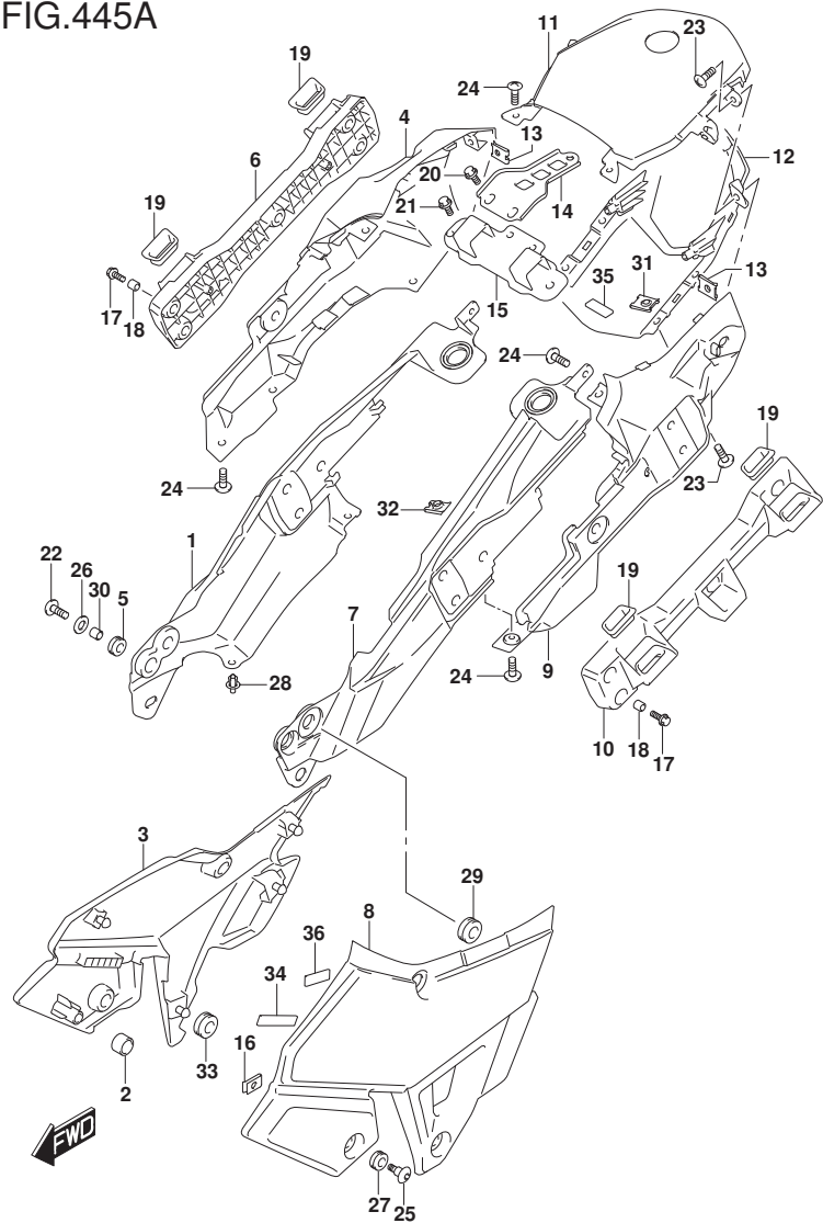
FIG.445A (1-E-5) FRAME COVER
